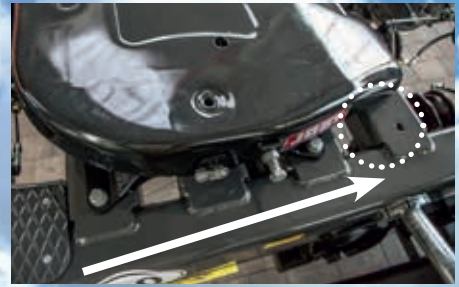
Mechanically adjustable fifth wheel plate for one-axle and tandem dolly
