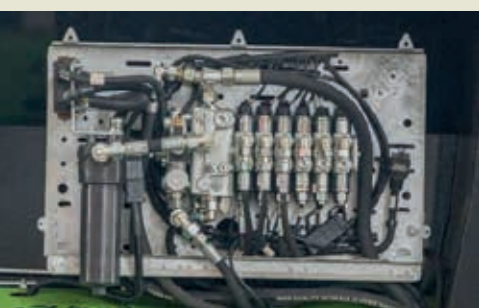
Control block with control panel for convenient operation
